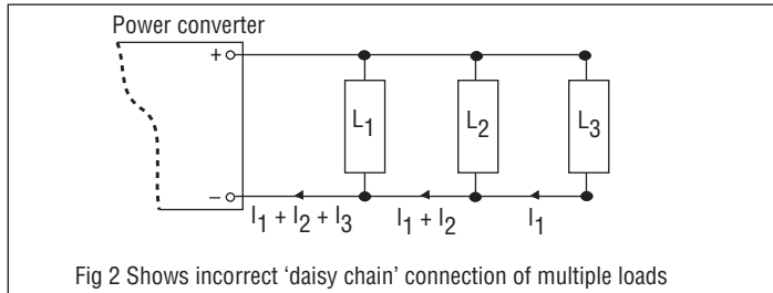
Fig 2 Shows incorrect 'daisy chain' connection of multiple loads
