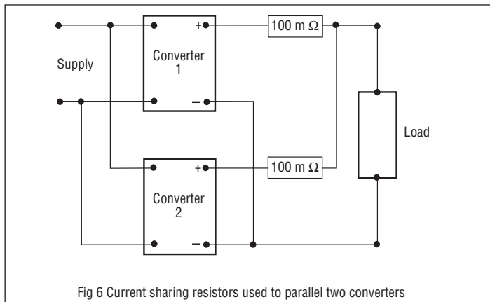
Fig 6 Current sharing resistors used to parallel two converters
